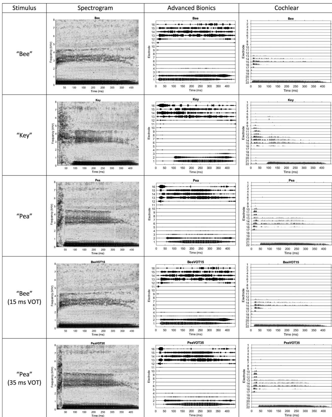
FIG. 3. Spectrograms of the five word tokens used in this study (second column). Simulated electrograms showing pulsatile stimulation patterns for the HiResolution F120 Sequential (HiRes F120S) processing strategy from Advanced Bionics (third column) and the advanced combinational encoder (ACE) processing strategy from Cochlear (fourth column). All electrograms were simulated using standard clinical maps. Electrode arrangement in the electrograms was based on ascending frequency from bottom to top of graph instead of the order of electrode numbers.
